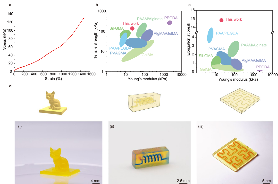
Extended Data Fig. 1 | The mechanical tensile properties and 3D printing results of the hydrogels prepared in this study. a , The stress–strain curve of the hydrogel. b–c , Ashby chart of the mechanical properties for various 3D-printed hydrogels, tensile strength versus Young's modulus ( b ) and elongation at break versus Young's modulus ( c ). Hydrogels include the hydrogel prepared in this work (red area), gelatin methacryloyl (GelMA) 35 , polyethylene glycol
