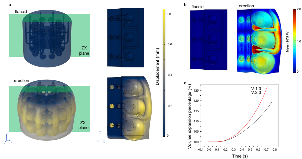
Extended Data Fig. 2 | Numerical simulation of the BCC models.
