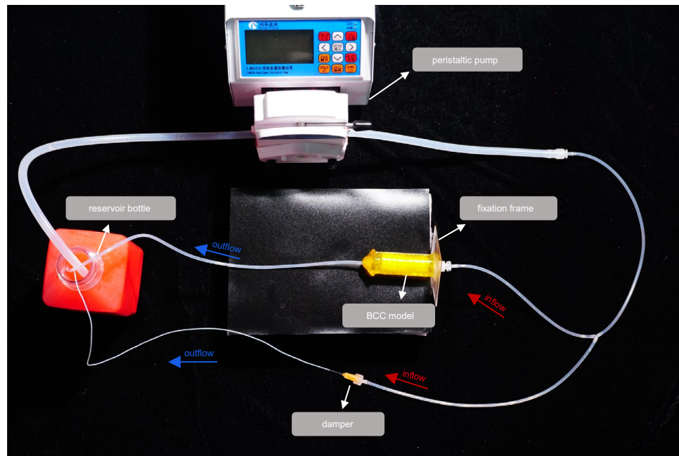
Extended Data Fig. 4 | Perfusion device for all the models (including the BCC, BCC with the wrapped biomimetic tunica albuginea, ED, and PD models). The fixation frame ensures that the model remains stable during perfusion.
