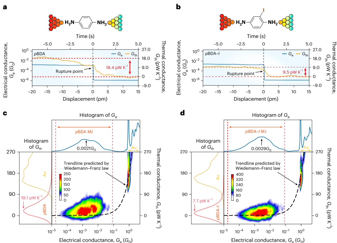
Fig. 3 | Analysis of thermal and electrical transport properties of single-molecule junctions. a, b, Averaged change in electrical ( G_e ) and thermal ( G_{th} ) conductances before and after the rupture of pBDA junctions (a) and pBDA-I junctions (b). c, d, 2D histograms constructed from ~1,500 measured G_e and
